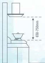
T-HOOD/ARCH-GLASS HOOD
