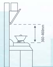
SLANTED HOOD
