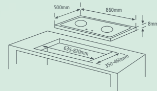
MBH-SD635 OPTIFLEX
