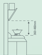
SLANTED HOOD
