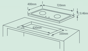
MBH-1665S
