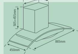
MDH-926MHC
