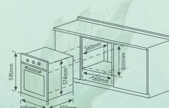
MBO-7680D
