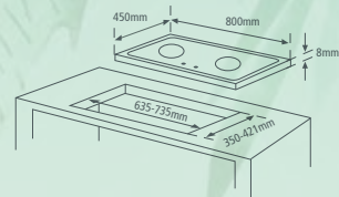
MBH-622 OPTIFLEX
