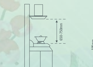
T-HOOD/ARCH-GLASS HOOD
